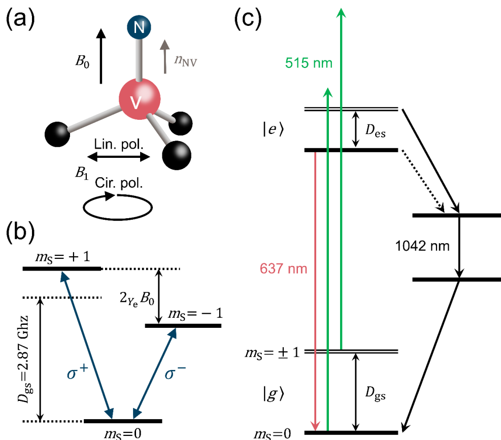
Figure 8 a) Schematics of an NV centre. b) Spin triplet ground state. c) Energy level diagram [56].
