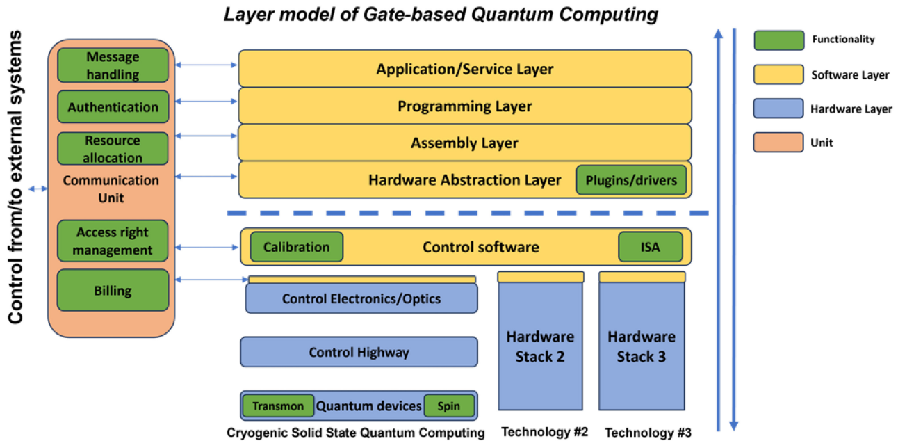
Figure 12 A possible break-down of software layers for quantum computing.
