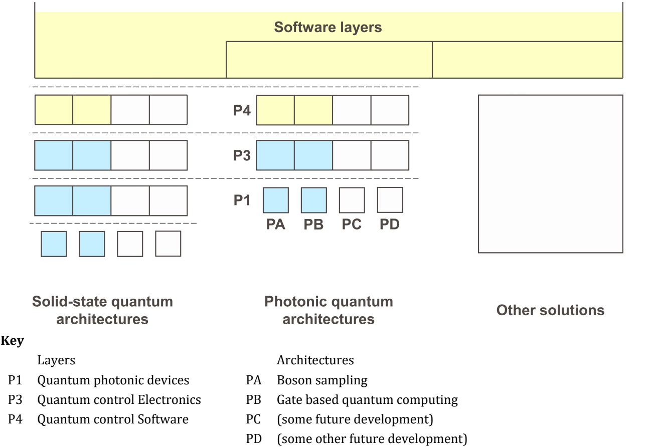
Figure C.1 A possible break-down into various modules for photonic quantum computing architectures
