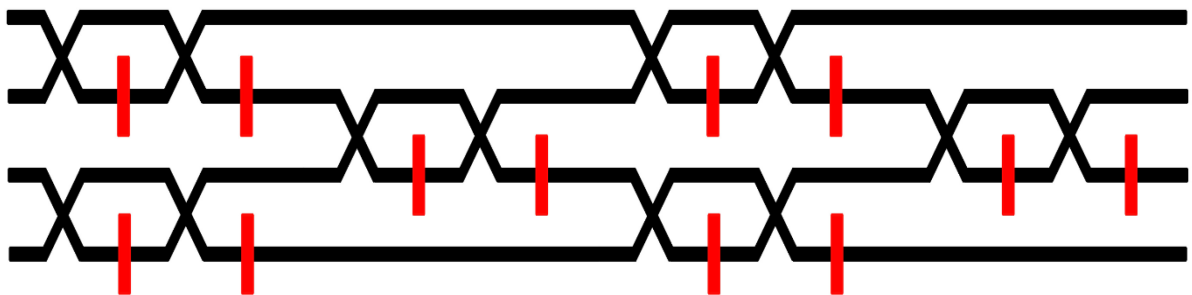
Figure C.3 An example network of a 4 mode quantum photonic processor. Six unit cells are combined using the architecture of Clements [113].
